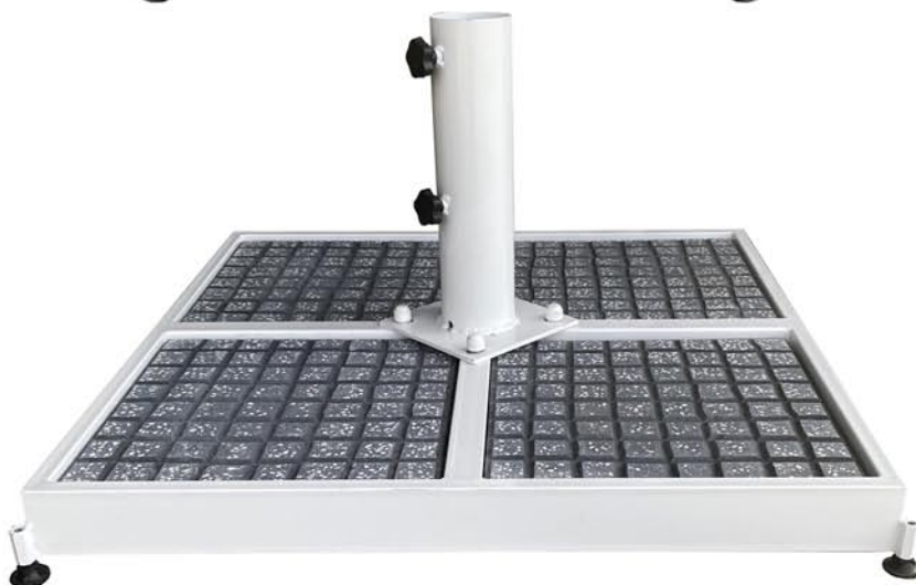
Art. A 1090 METAL BASE, for concrete slabs 40x40 cm, for parasol pole \Phi 60-90 mm size 88x88 cm, (concrete slabs not included).
