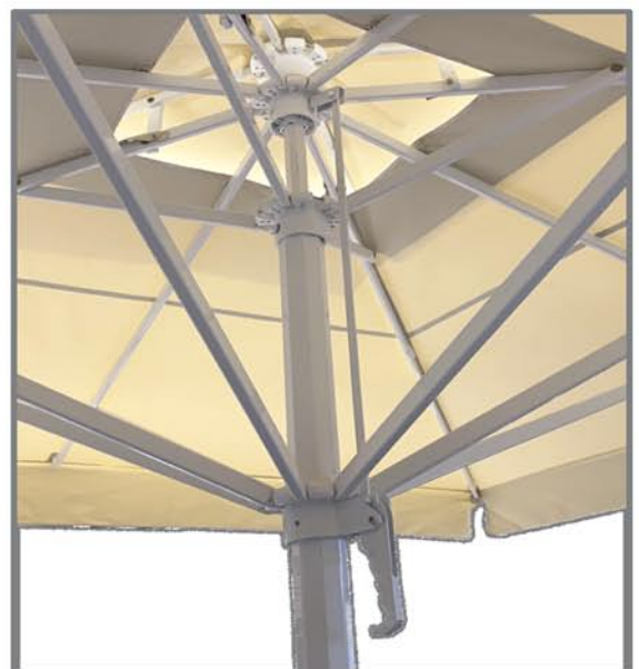
internal structure
