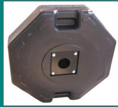
Art. BC 2035 concrete base with plastic cover,, octagonal 55 Kgr. for pole \Phi 60 mm.
